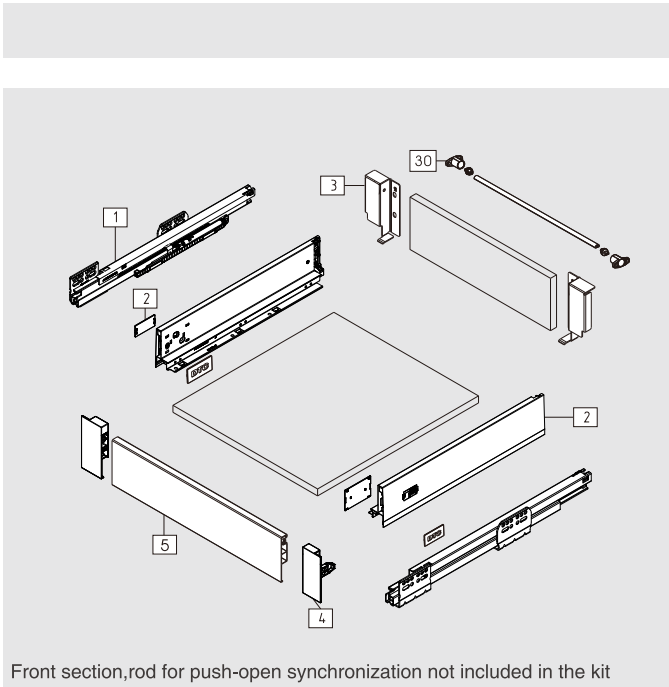
Front section,rod for push-open synchronization not included in the kit
